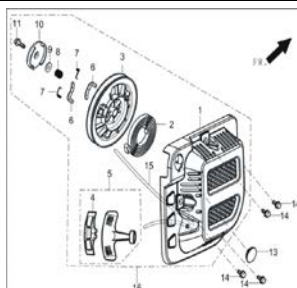
FIG.7 STARTER,RECOIL ( E07 )
